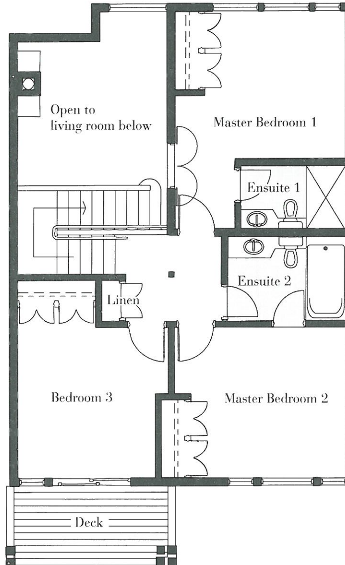
Second Floor
