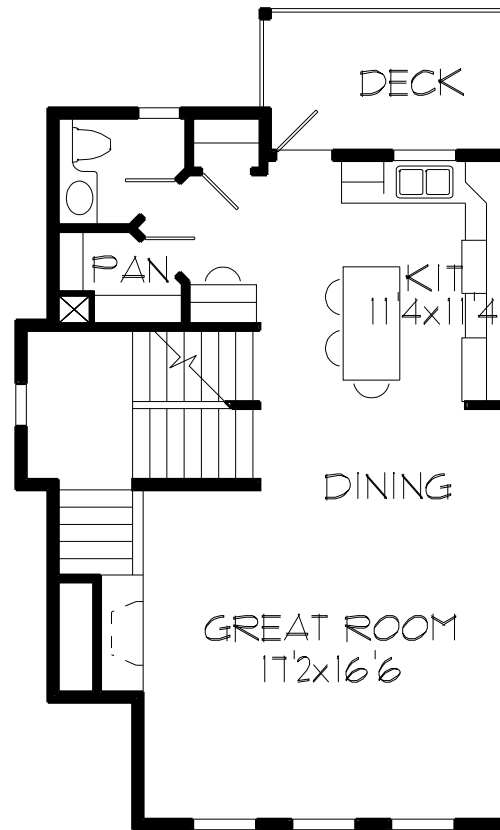
UNIT A MAIN FLOOR PLAN 710 SQ.FT. 1646 TOTAL SQ.FT.
