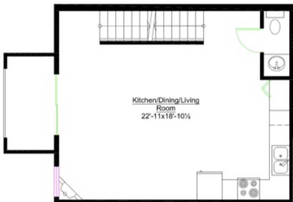
SECOND FLOOR
