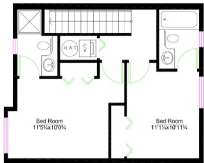
THIRD FLOOR
