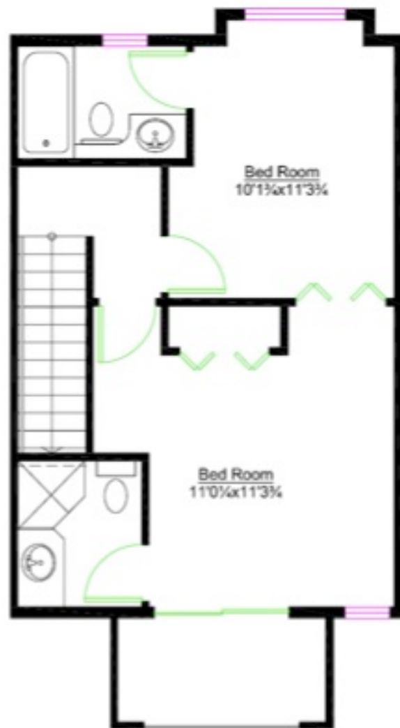
THIRD FLOOR
