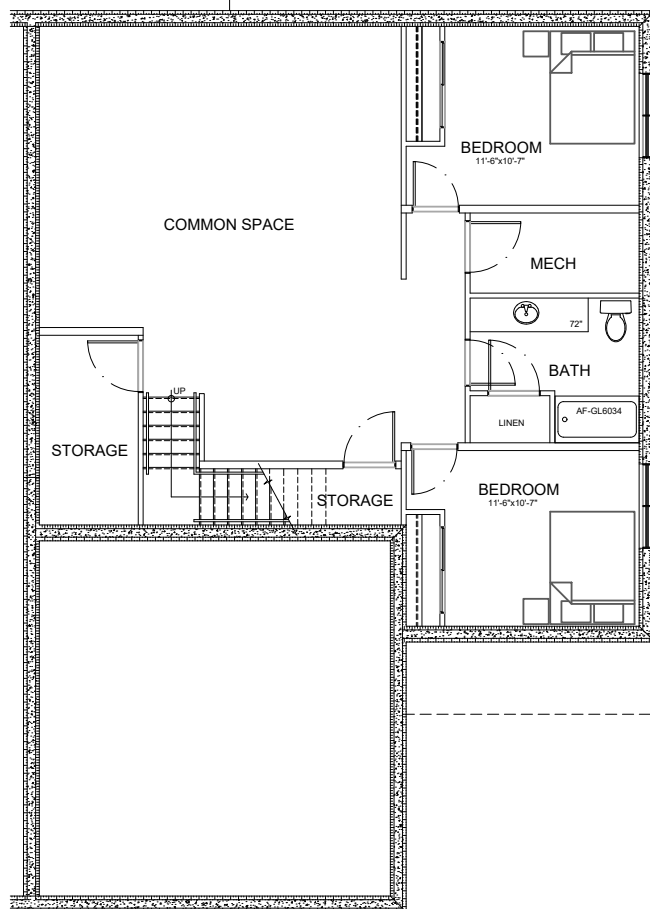
BASEMENT – 1225 SQ FT
