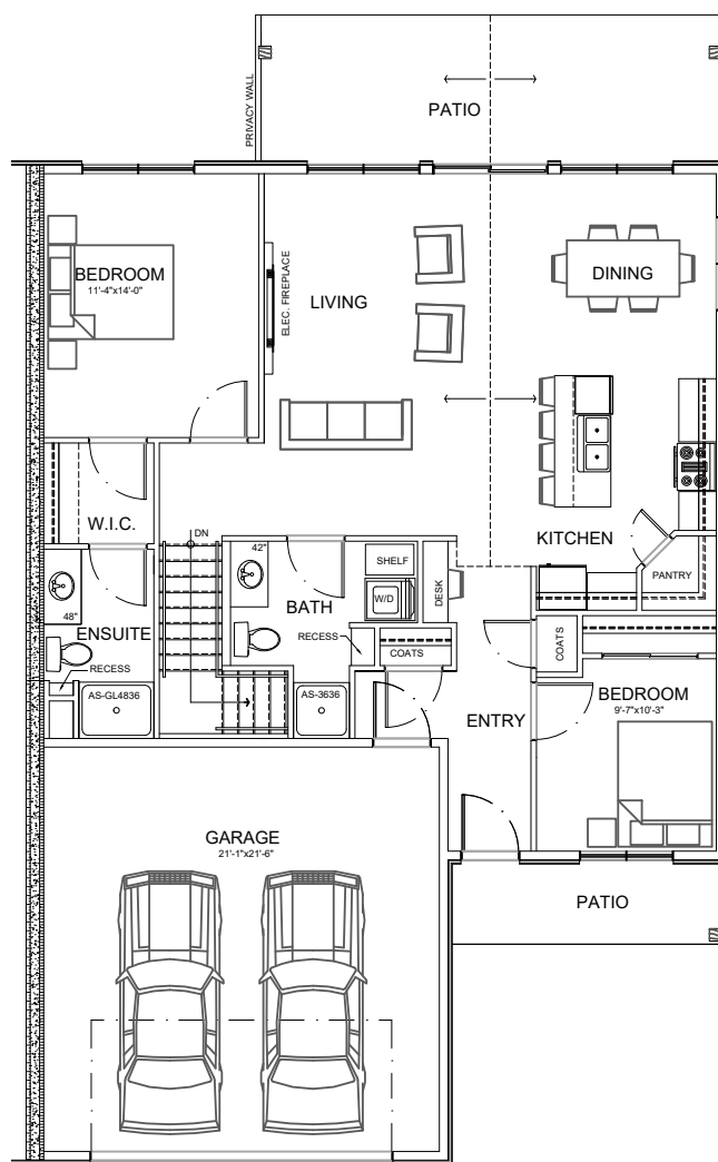
MAIN FLOOR – 1225 SQ FT
