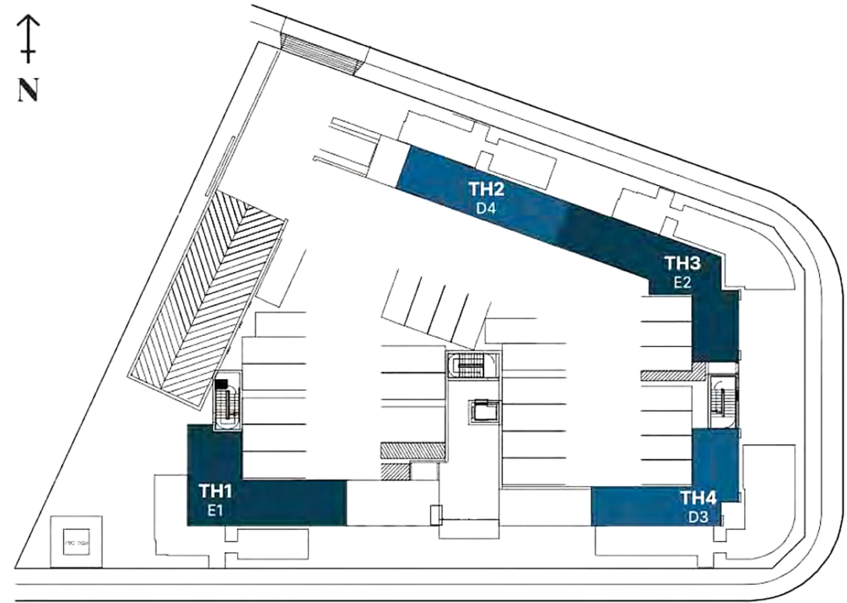
GROUND FLOOR
